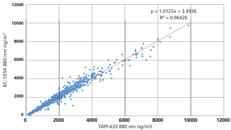
Figure 4: 10 Wavelength Comparison
